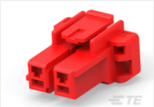
TE Part #1-1376388-3 5.0 PK CONN. 2P PLUG HSG (W/O GF) - RED
