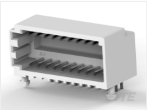
TE Part # 1-292138-8 CT DOUBLE ROW ASSY H 18P HDR N
