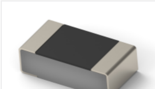
TE Part #1-2176467-9 TLRP 1206 1.0W R030 1% 75PPM 5K RL
