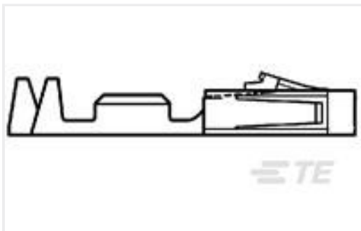
TE Part #104481-6 SHORT POINT RECP CONT LP
