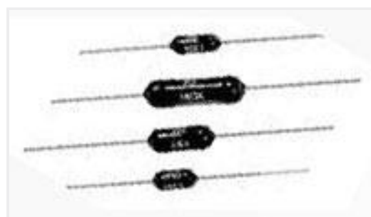
TE Part #7-1879664-9 H8 7K5 0.1% 15PPM
