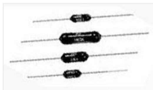
TE Part #6-1879665-0 H8 51K1 0.1% 15PPM
