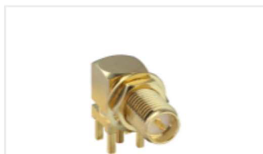
TE Part #CONREVSMA002-L-G RP-SMA RA Jack 50 Ohm PCB Through Hole
