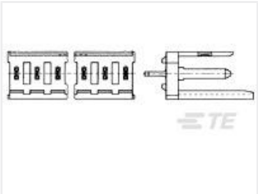
TE Part #280616-1 4P MOD 1 P.S.ASSY.
