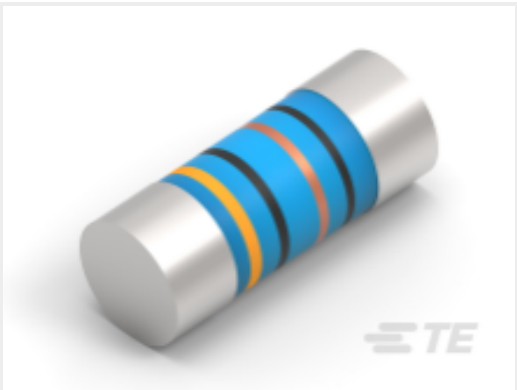
TE Part #8-2176316-3 MELF SMA-A 33R 1% 50PPM 0207 1W
