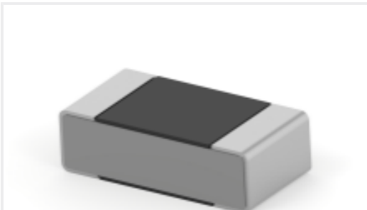
TE Part #4-1879129-5 RN 0402 1K69 0.1% 10PPM 5K RL
