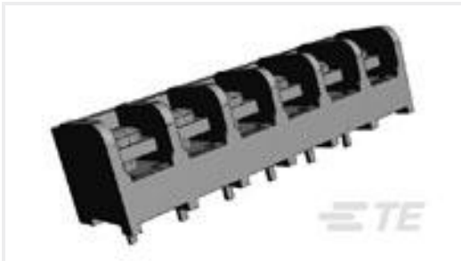
TE Part #1-1674231-1 2.5MM PITCH BATTERY REC ASSEMBLY DIP TYP
