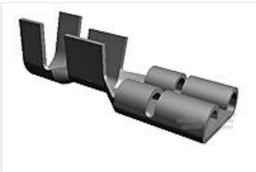
TE Part #444335-1 250 FASTON REC 16-14 AWG BR
