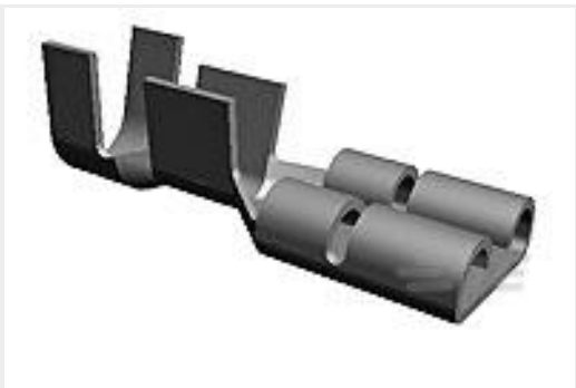
TE Part #444334-1 250 FASTON REC 22-18 AWG BR
