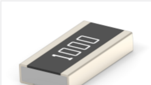
TE Part #1-2176558-1 3430 B2 1% 2R4 100ppm 1k RL
