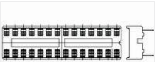
TE Part #1-2199298-8 24P,DIP SKT,300 CL,LDR,PB FREE
