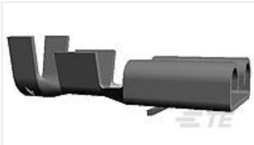
TE Part #5-160446-2 FF 250 REC 1.0-2.5MM2 TPPB
