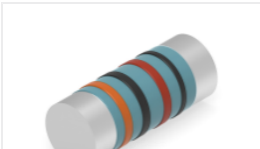
TE Part #1879283-4 MELF SMA 82K 5% 100PPM 0.5W 0207
