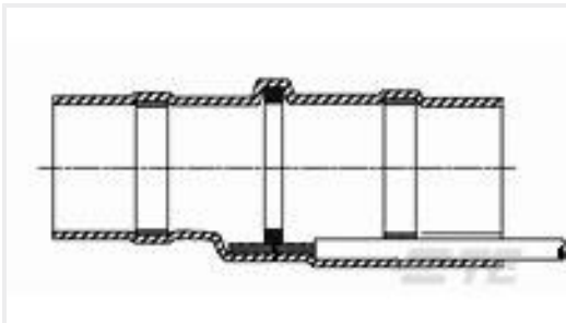
TE Part #F80290-000 B-155-4174-35-22-5/9-10
