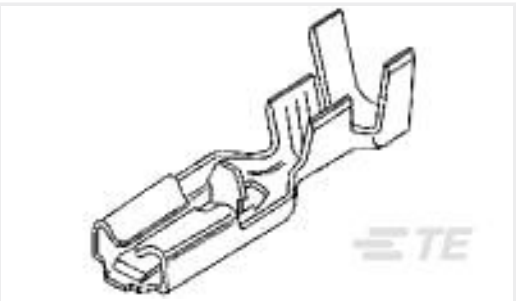
TE Part #63313-1 PL 187 RECEPTACLE 20-16 AWG TPBR
