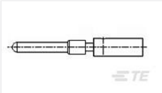
TE Part #5-1437720-4 T01-CRIMP-P03
