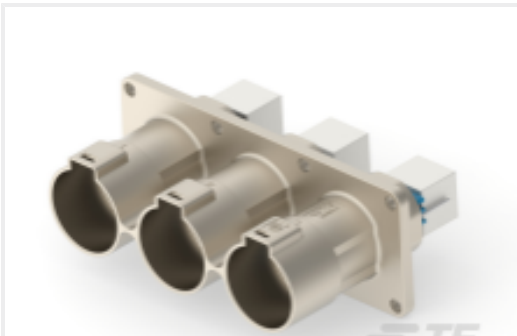
TE Part #2-2399608-1 3POS,HVP1400,ASSY,180DEG,COD A /B/C
