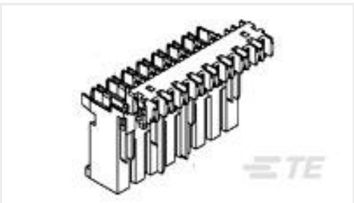
TE Part #1-293003-5 MONO SHAPE TAB CONNECTOR 5 POS
