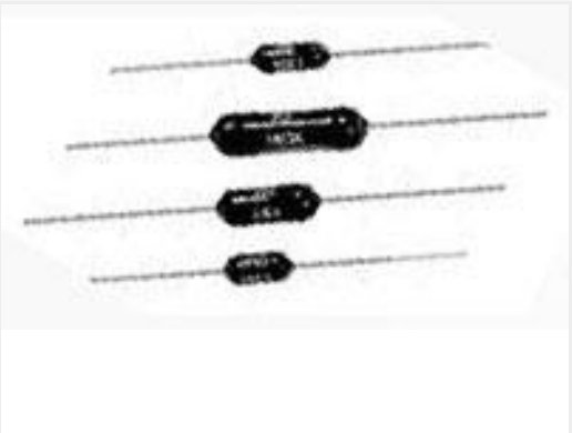
TE Part #4-1879663-6 H8 316R 0.1% 15PPM
