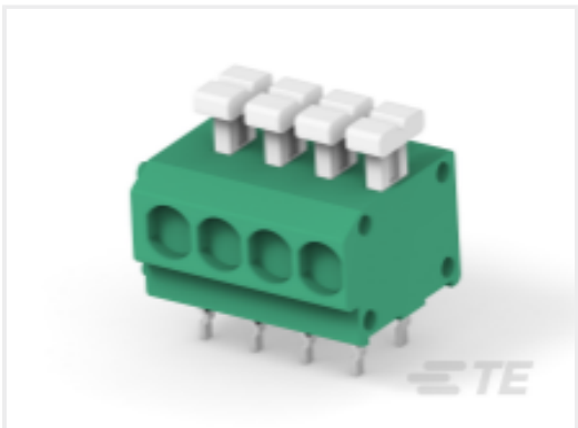
TE Part #1-2834017-4 4POS 3.81MM TEPS CONN.
