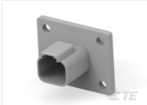
TE Part #DT04-2P-L012 REC, 2P, GRY, N, FLANGE
