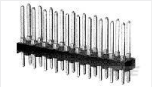
TE Part #87227-4 08 MODII HDR DRST UNSHRD .100
