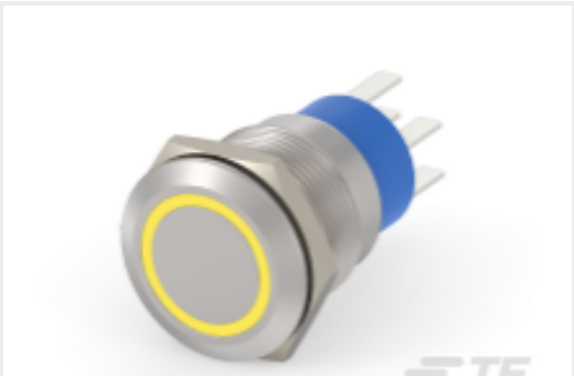
TE Part #5-2213764-1 AV19 DPM 3A FIX RING LED YELLOW 24V
