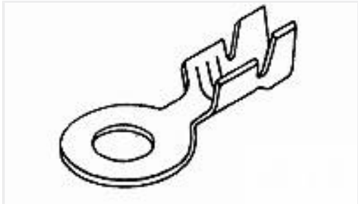
TE Part #62691-2 RING 12-10 AWG TPBR
