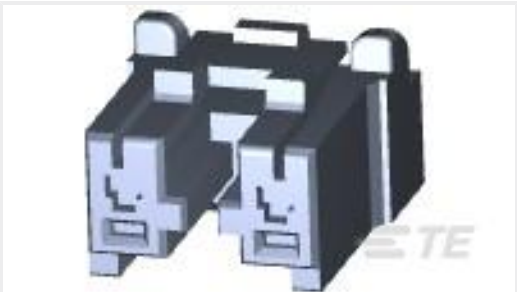
TE Part #1747050-1 GRACE INERTIA CONNECTOR 7.92 2POS PLUG H
