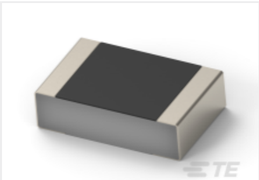
TE Part #2176451-1 CPF 0201 49R9 0.1% 25ppm 1K RL
