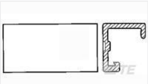
TE Part #1-640550-8 18P MTA100 COVER
