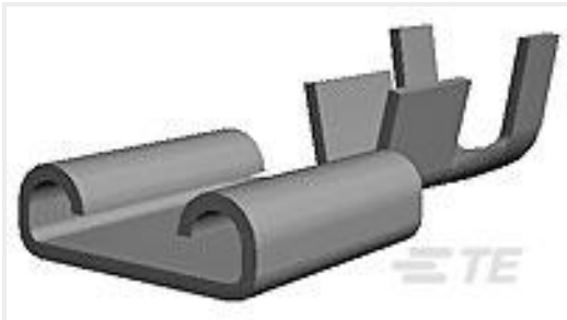
TE Part #62428-3 250 FASTON REC 12-10 AWG TPBZ
