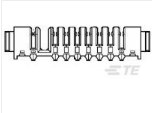
TE Part #1717620-1 2.5MM PITCH BATTERY REC. ASSY 8POS. R/A
