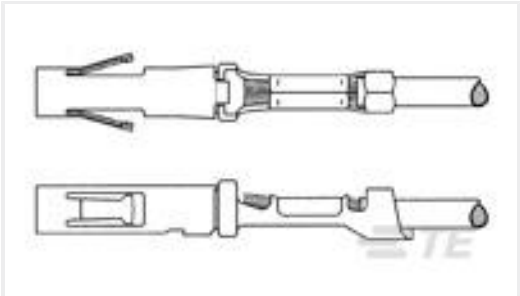
TE Part #164153-6 CONTACT, SOCKET, CRIMP, TYPE XI
