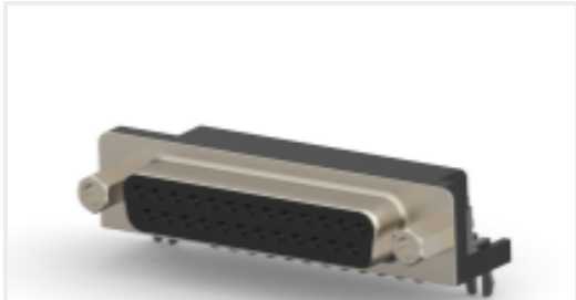
TE Part #2311766-1 AMPL REC, HD20, R/A, 25P, S/L, .318
