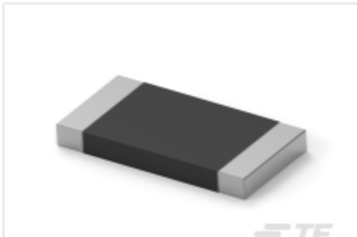
TE Part #6-2176421-6 TLRP 2512 2.0W R075 1% 50PPM 4K RL
