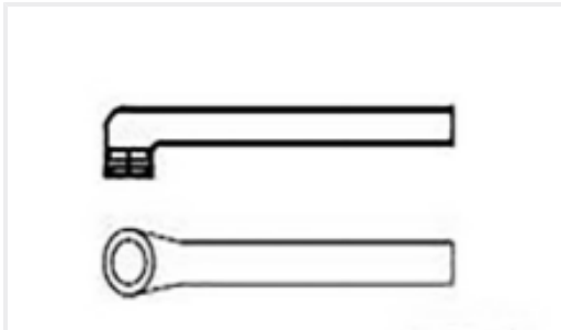
TE Part #CAT-R21-731055 Low Profile Heat Shrink Boots: Poly Mold, Lipped, Right Angle
