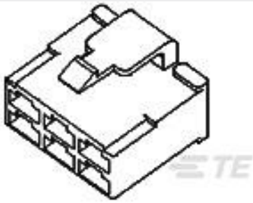
TE Part #172134-2 FF 250 PLUG HSG 4P NYLON BLACK
