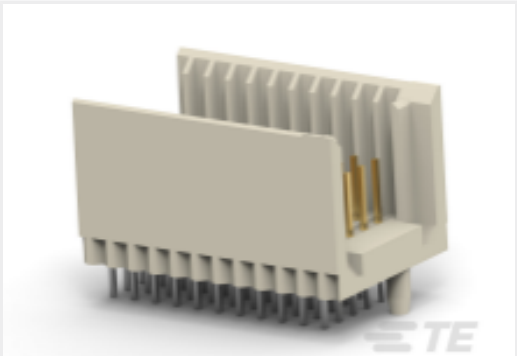
TE Part # CAT-472-Z12 Hard Metric Male Connector: Traditional Backplane, Mezzanine, 2mm
