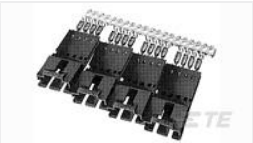
TE Part #103944-1 8X2 MTE SHRD PIN SR POL .100CL
