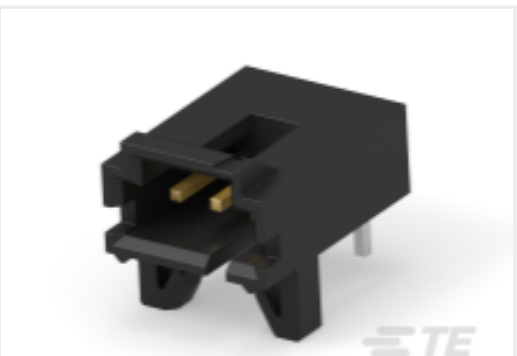
TE Part # 103673-2 03 MTE HDR SRRA LATCH W/HLDWN
