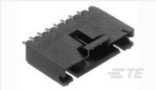
TE Part # 103638-9 10 MTE HDR SRST LATCH .100CL
