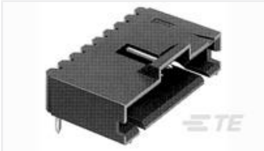
TE Part # 103635-9 10 MTE HDR SRRA LATCH .100CL
