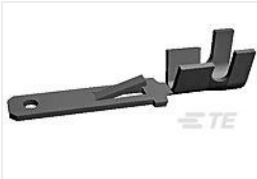
TE Part #42460-2 FF 250 TAB 18-14AWG TPBR
