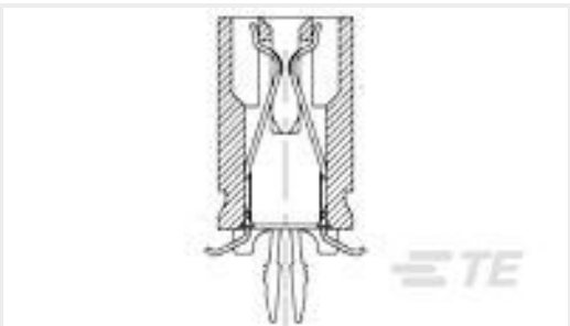
TE Part #5145113-1 CONNECTOR ASSEMBLY, DUAL POSIT
