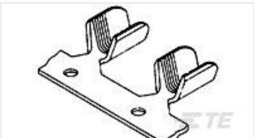
TE Part #63621-2 SPLICE S-MINI/AMVAR 0098TPCUBR
