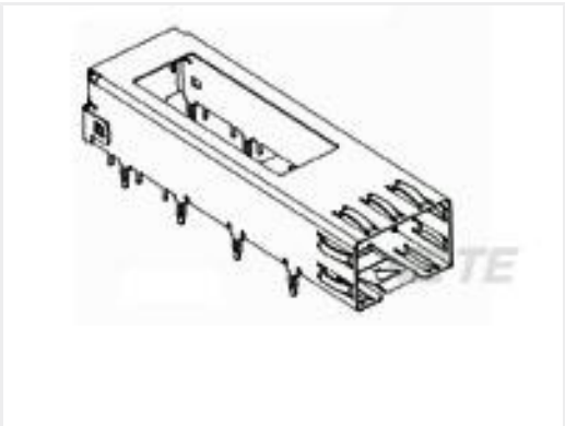
TE Part #2227316-1 DWDM Cage Assembly, 11 PF
