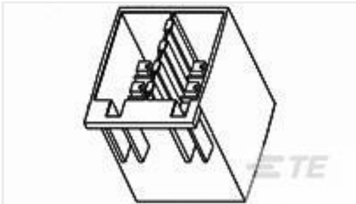
TE Part #338696-1 FASTIN FASTON (FF) HOUSING TAB
