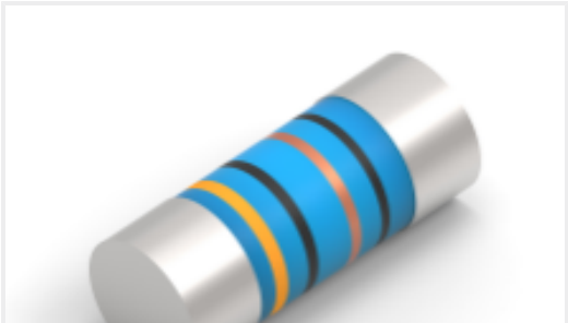
TE Part #5-2176315-8 MELF SMA_A 4K7 1% 50PPM 0204 0.4 W
