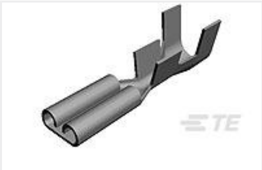
TE Part #181902-1 250 FASTON,REC.,24-17 AWG,TPBR
