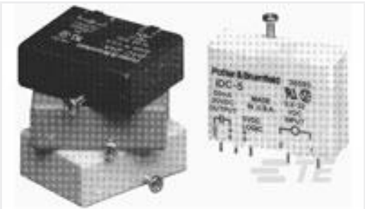
TE Part #2-1393028-4 OAC-24 = PCB MOUNT,3A,120V AC - DC I/p
