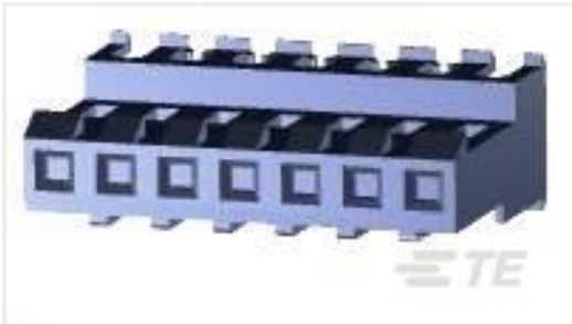
TE Part #3-640599-7 07P MTA156 CONN ASSY 18AWG ORA
