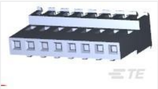
TE Part #3-640604-8 08P MTA156 CONN ASSY 18AWG LF
