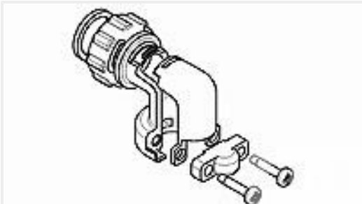
TE Part #1546350-2 R/A CABLE CLAMP KIT,SZ 23,CPC
