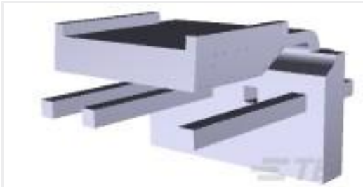
TE Part #3-644661-4 04P MTA156 HDR ASSY POL W/O#2
