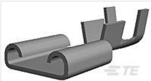
TE Part #6-160432-3 250 FASTON REC 20-16 AWG NPST
