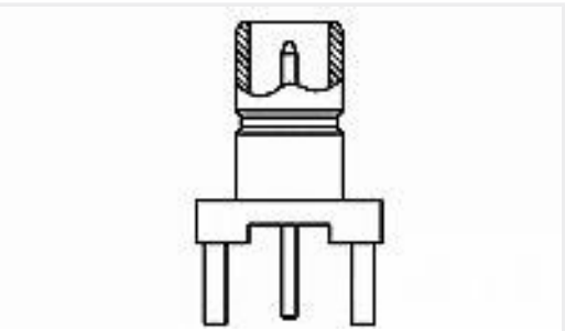
TE Part #415504-4 JACK,PCB,MINI-SMB VERT 75 OHM
